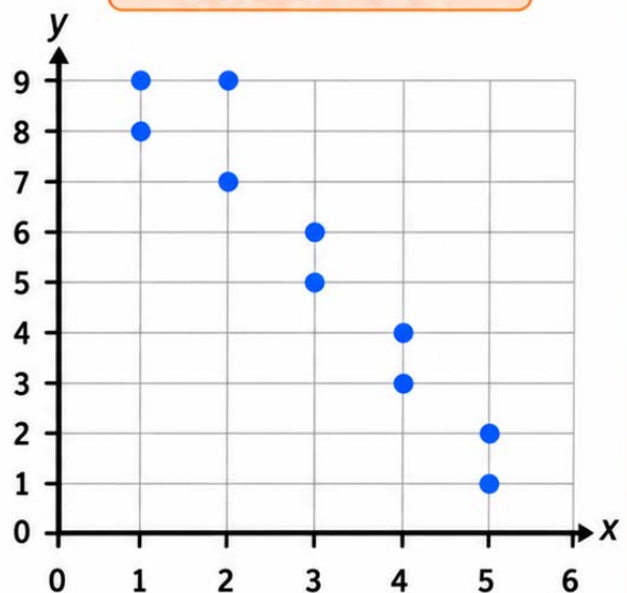
Scatter Plot 4
