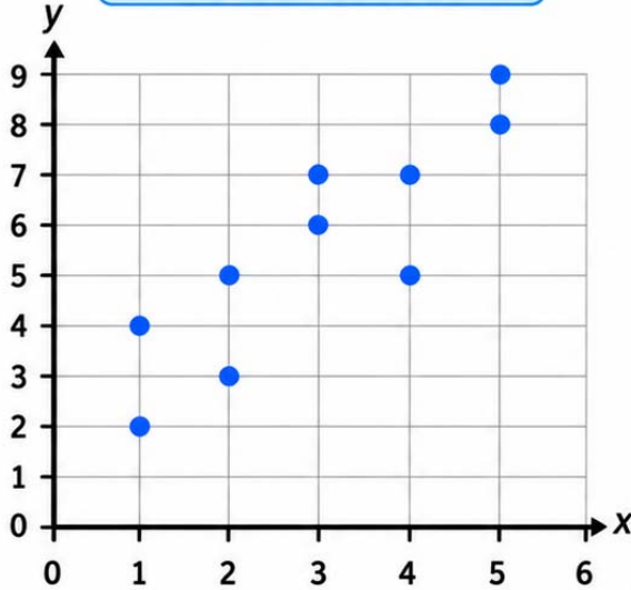
Scatter Plot 1
