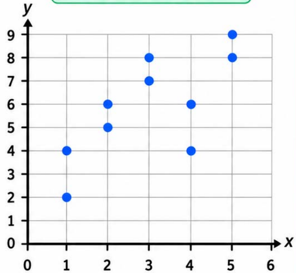
Scatter Plot 3
