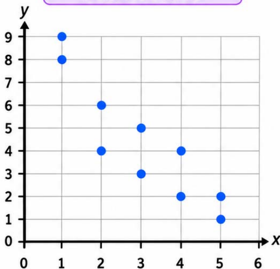
Scatter Plot 2
