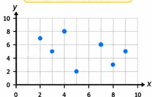
Scatter Plot 5
