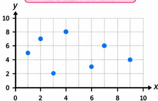
Scatter Plot 3
