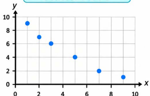
Scatter Plot 6
