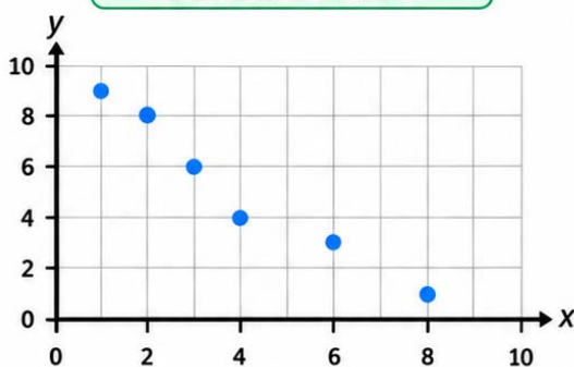
Scatter Plot 2
