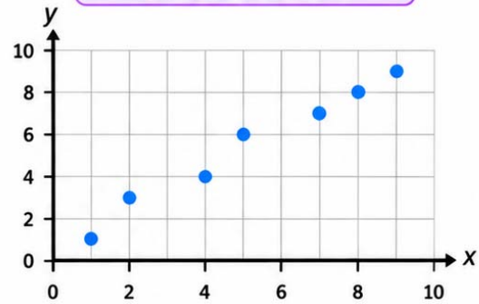
Scatter Plot 4
