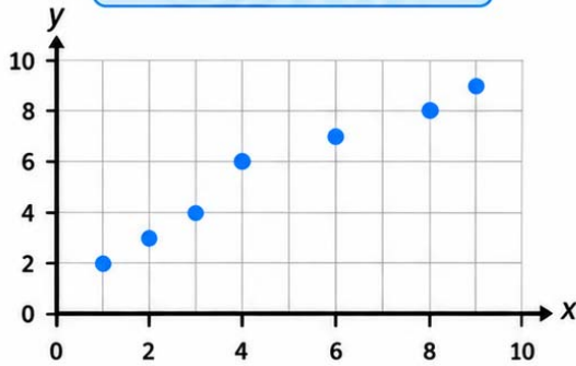
Scatter Plot 1
